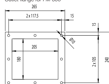
Outlet flange for FM 600
