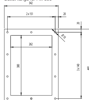
Outlet flange for FM 800
